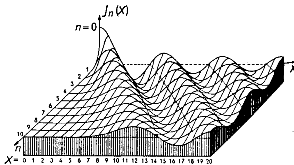
Fig. 2. Illustration of Bessel functions. (Reproduced by kind permission of the publishers from Tables of Functions by Jahnke & Emde. New York: Dover Publications.)
