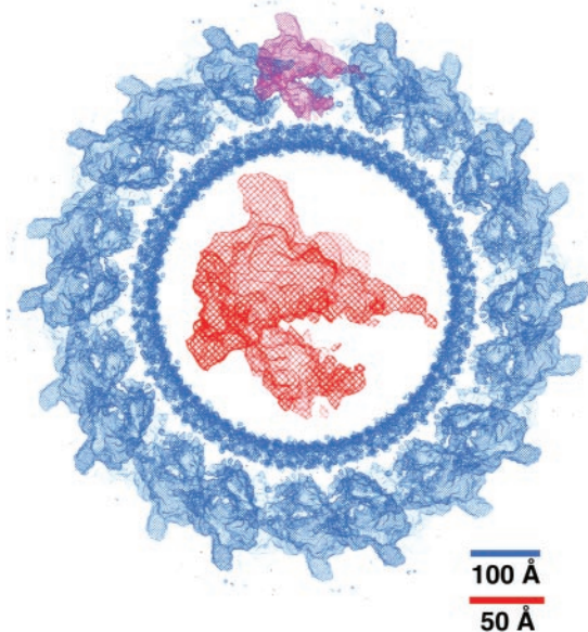
Fig. 2. Cryo-EM structure of E. coli core RNAP. Shown in blue is a 200-Å thick cross section through the reconstructed tube, contoured at 1.1\sigma . The noisy, inner circle of density is caused by the cylindrical lipid bilayer. Arranged around the outside of the lipid tube are the E. coli core RNAP molecules. The density caused by a single E. coli core RNAP molecule is highlighted in purple. The density for a single E. coli core RNAP molecule, extracted from the whole reconstruction and magnified, is shown in red in the middle of the cross section. Scale bars are for the whole reconstruction (blue) and magnified molecule (red).
